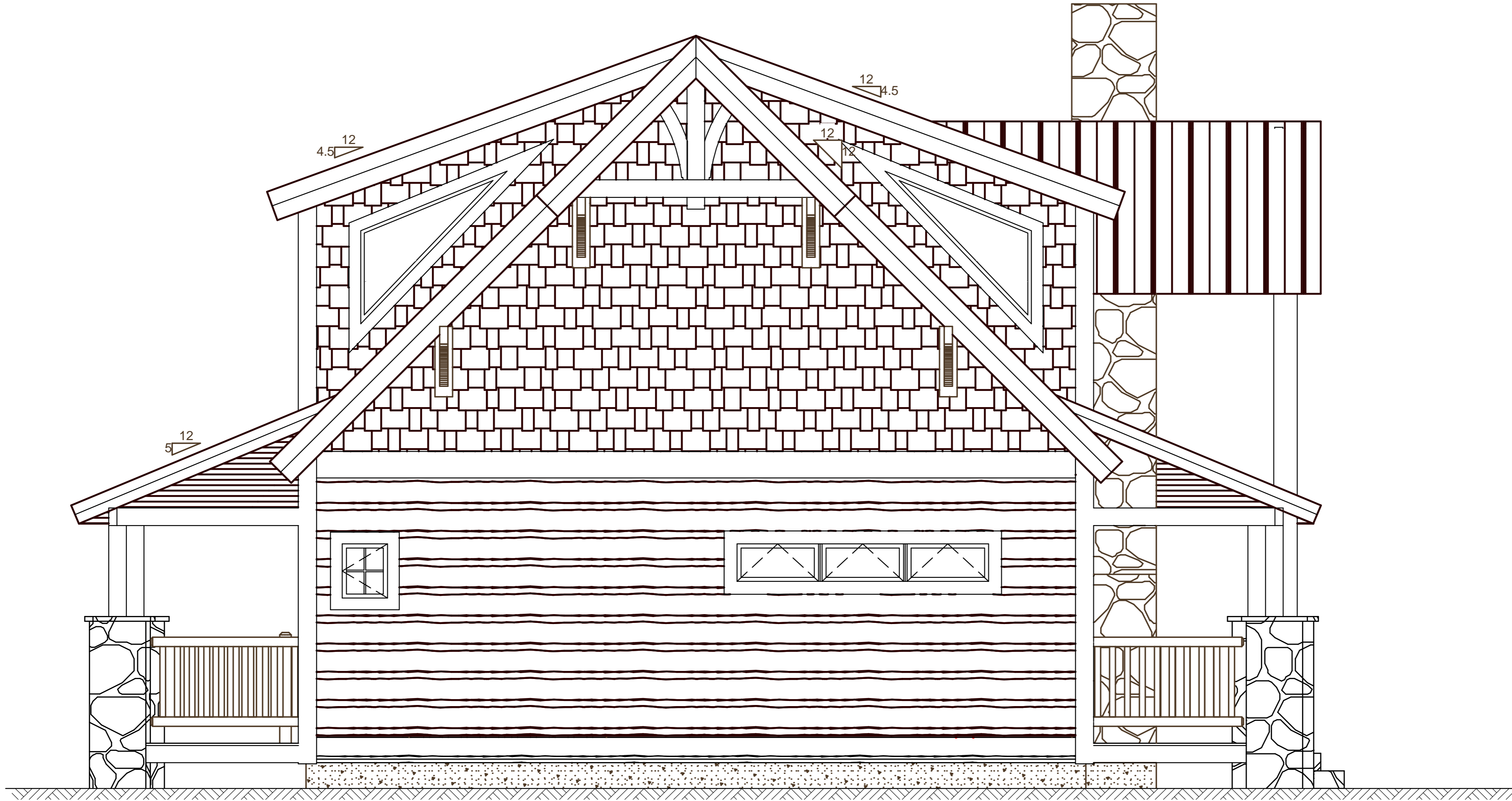
LEFT ELEVATION NOTE: GRADE CONDITIONS TO BE VERIFIED ON SITE
