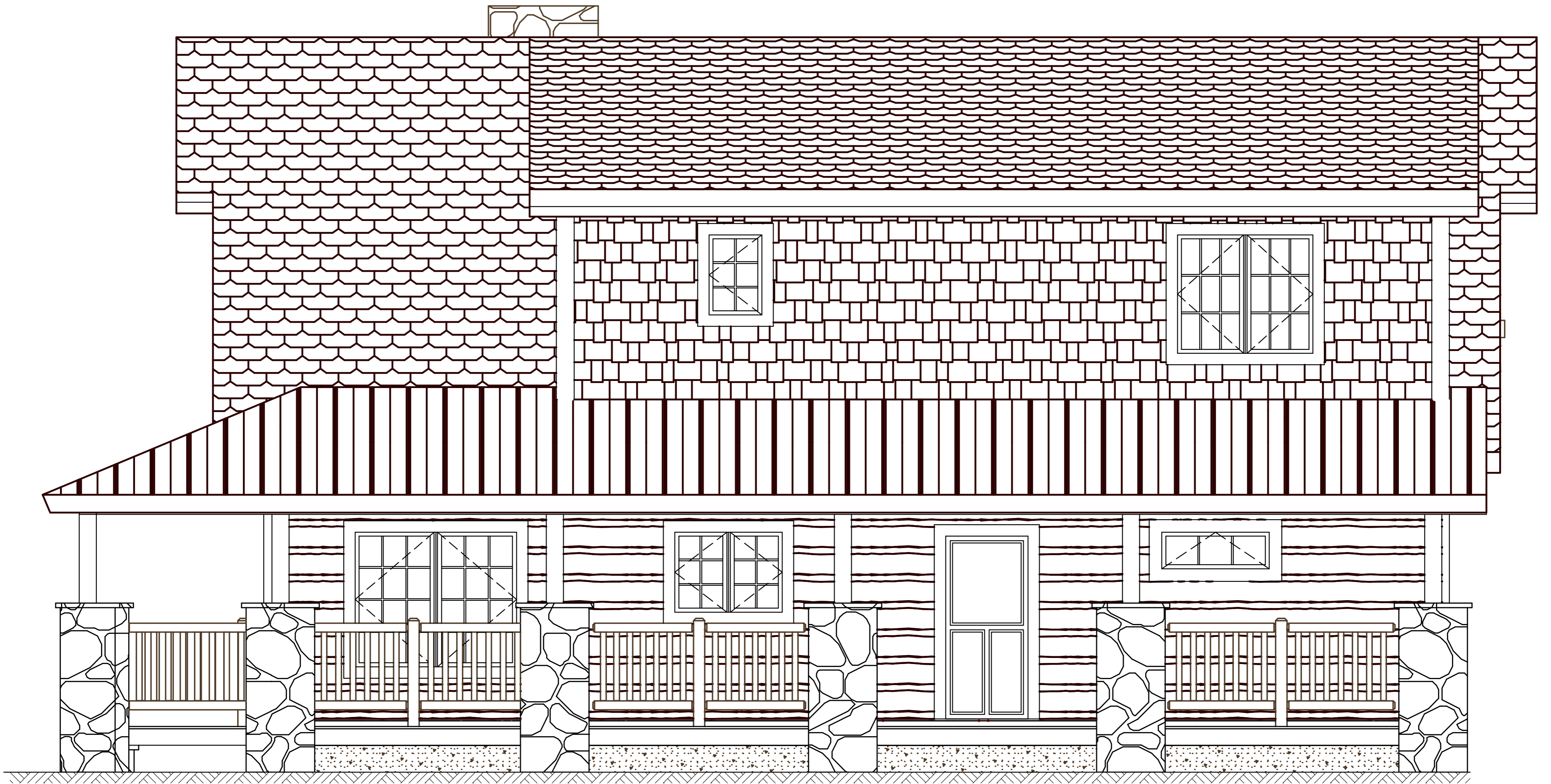
REAR ELEVATION
