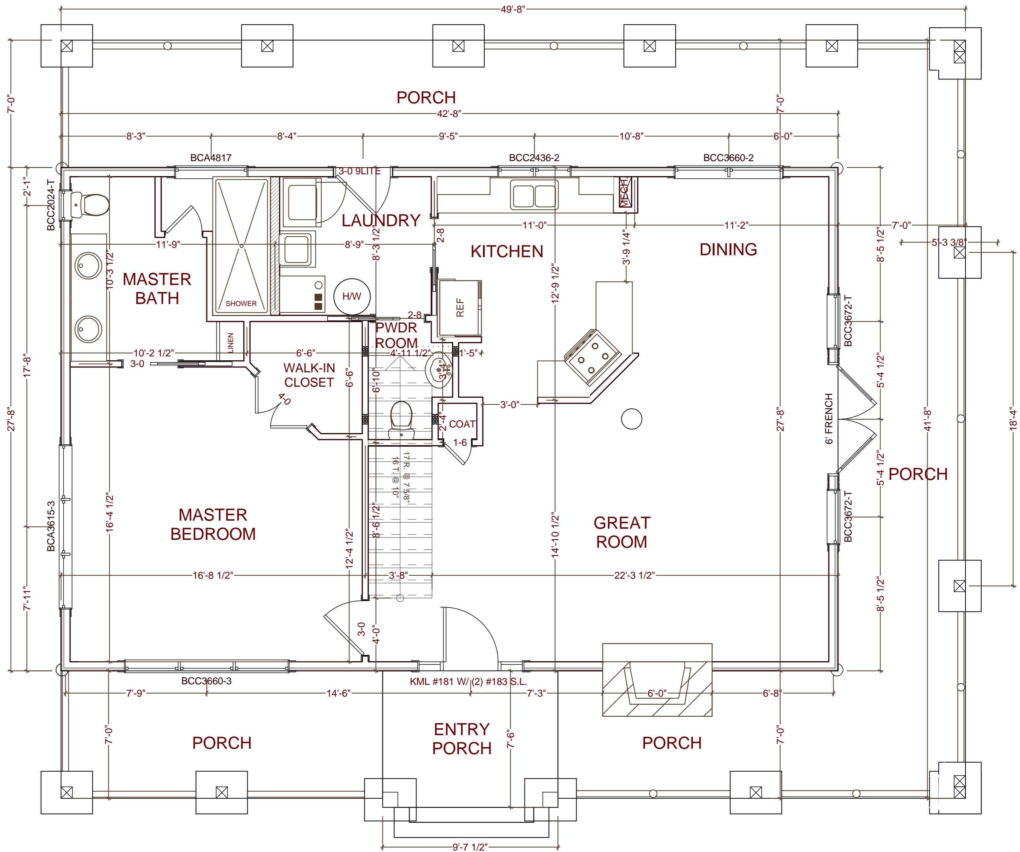
MAIN FLOOR PLAN
